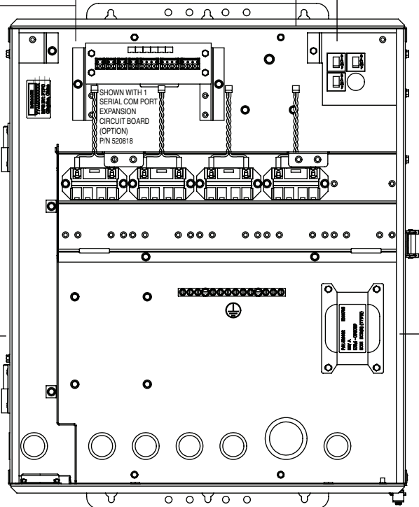
EasyTouch PL4/PSL4 Control System Power Center (Front panel and outdoor control panel not shown)
